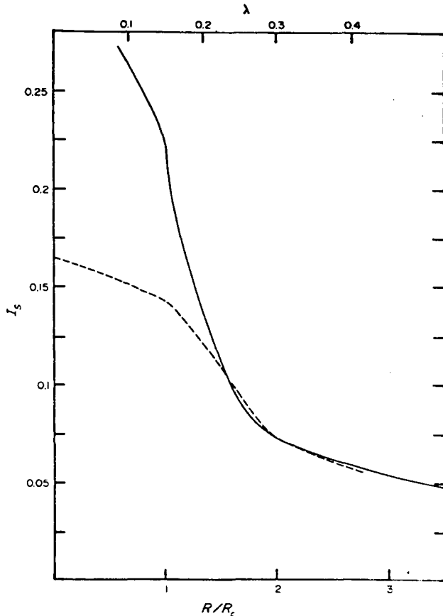
Fig 6 Calculated Static Impulse vs Dimensionless Radius for Detonation (solid line) and Deflagration (dashed line) of Large Hydrogen-Oxygen Charge
