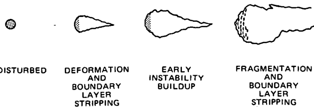
Fig 17 Phenomena Associated With Breakup of Fuel Drops in a Two Phase Detonation (from Ref 5)
