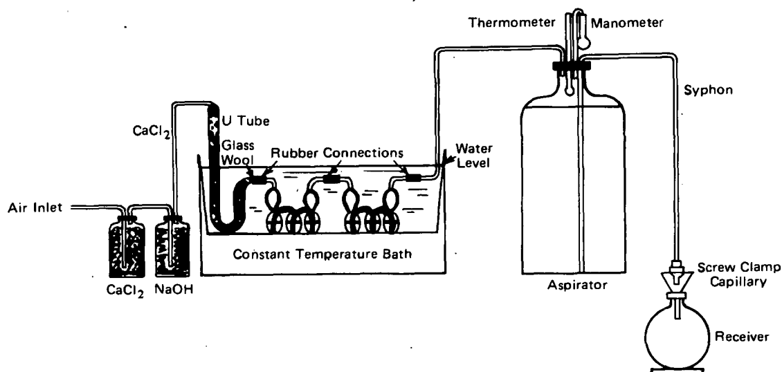
Fig 1 Weight Loss Measurement Technique
